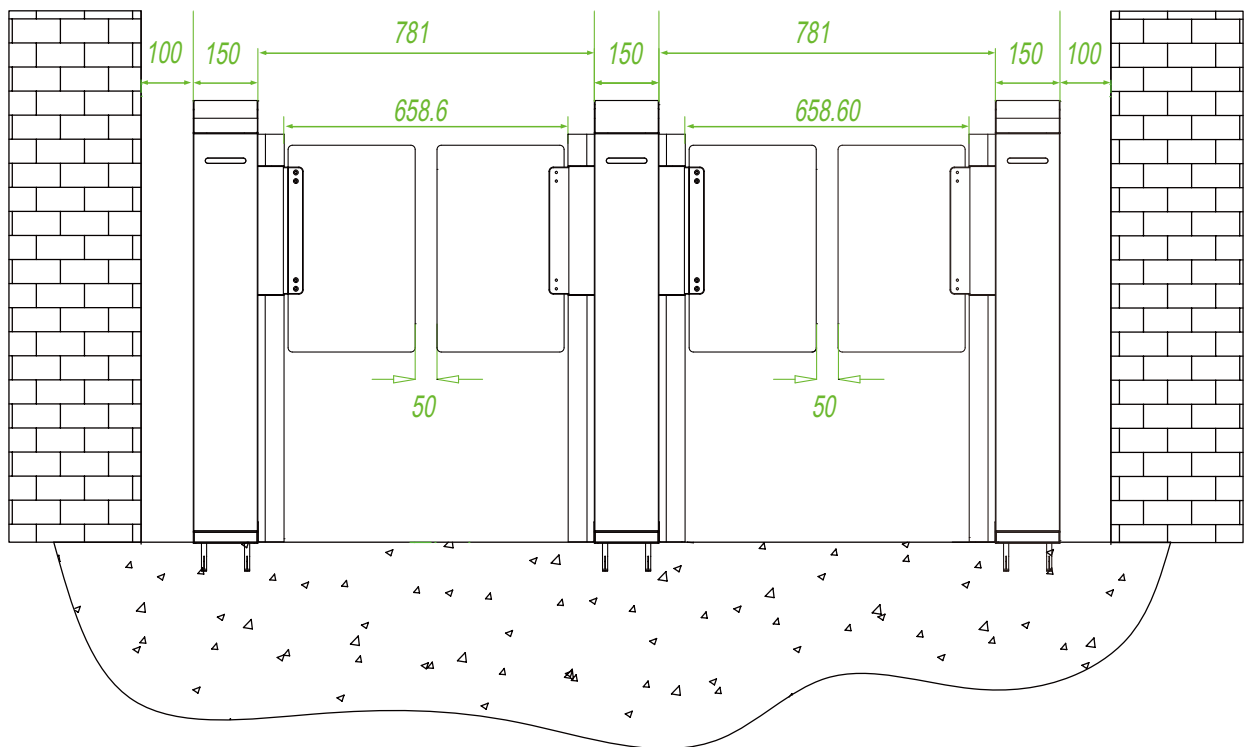
Figure 1-1 SBTL7000 Series Dual-lane
